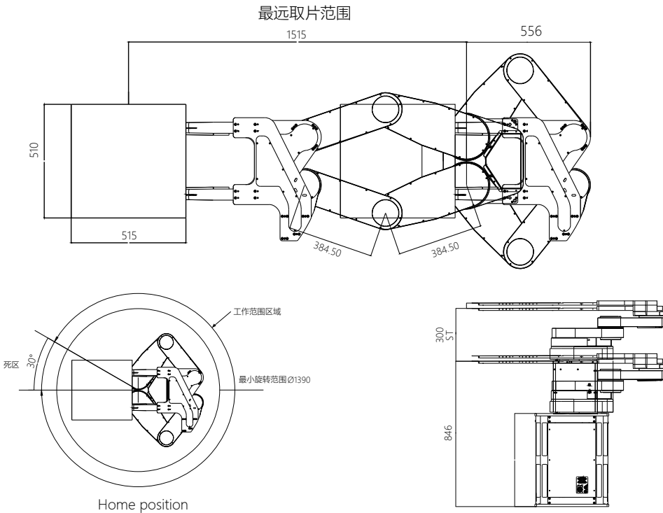
双臂机械臂运动范围示意图 Schematic diagram of the motion range for a dual-arm robotic arm
